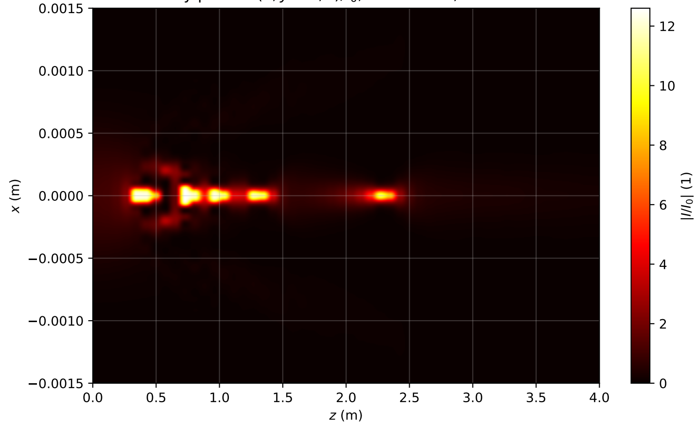
Intensity profile I(x, y = 0, z)/I_0 , \text{Pin}=9.0\text{Pcr} , artificial time
